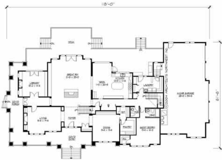
MAIN FLOOR - PLAN M6575A4S-0 MAIN FLOOR: 3406 S.F. GARAGE: 1472 S.F.
