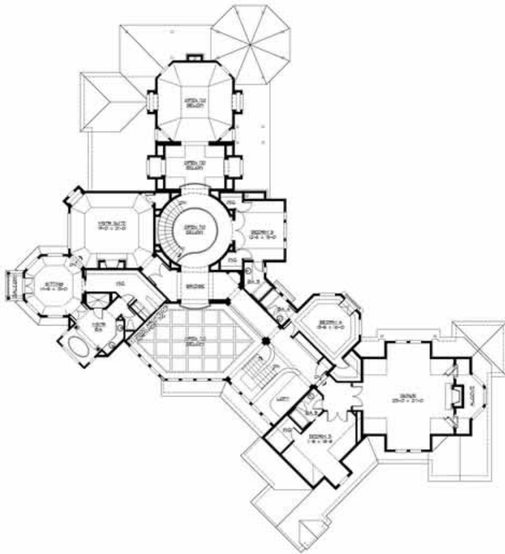
UPPER FLOOR - PLAN M7400A45-2 SCALE 1/4" = 1'-0"
